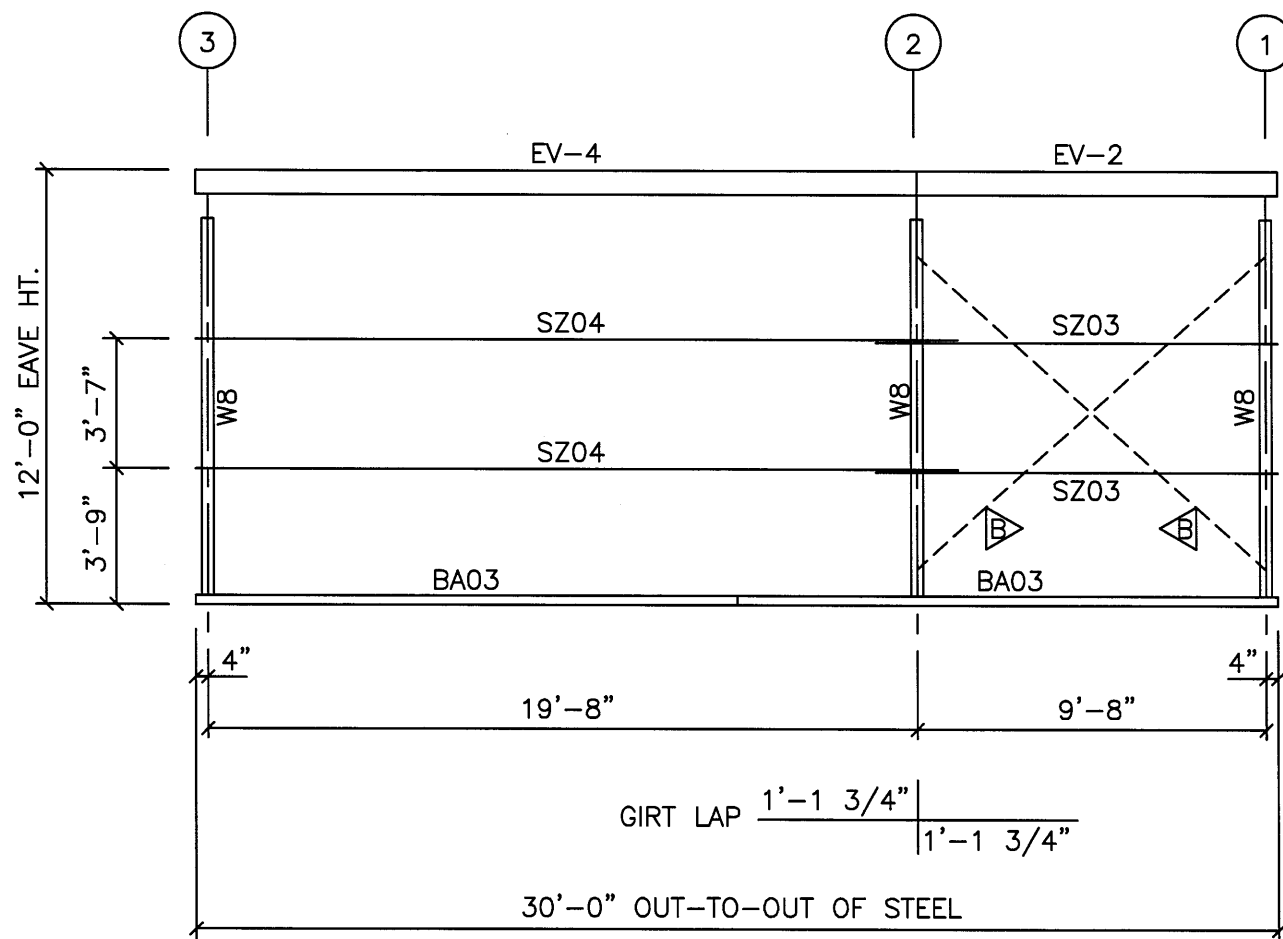
SIDEWALL FRAMING ELEV. @ COL. LINE B N.T.S.
