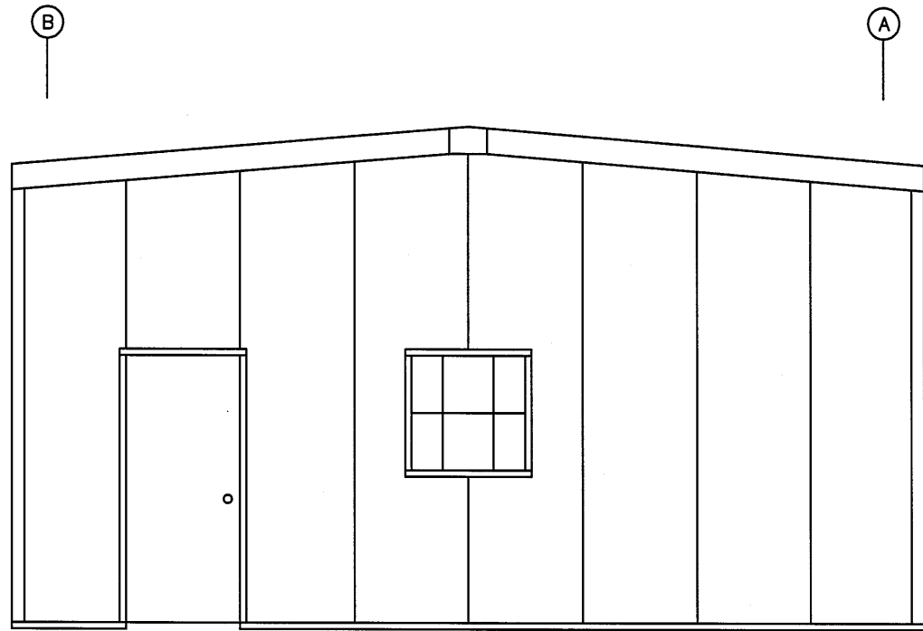
ENDWALL SHEETED ELEV. @ COL. LINE 1 N.T.S.
