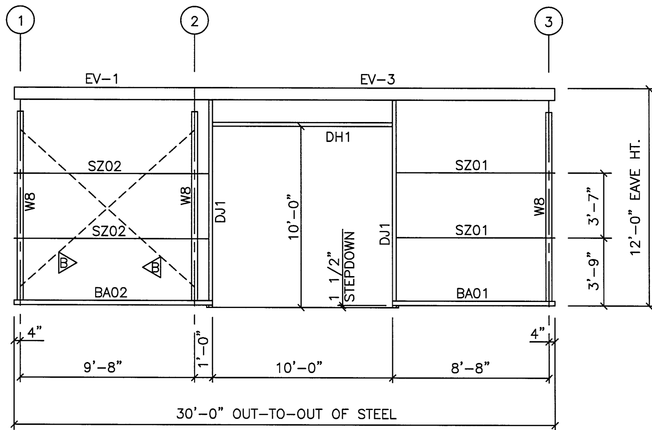
SIDEWALL FRAMING ELEV. @ COL. LINE A N.T.S.
