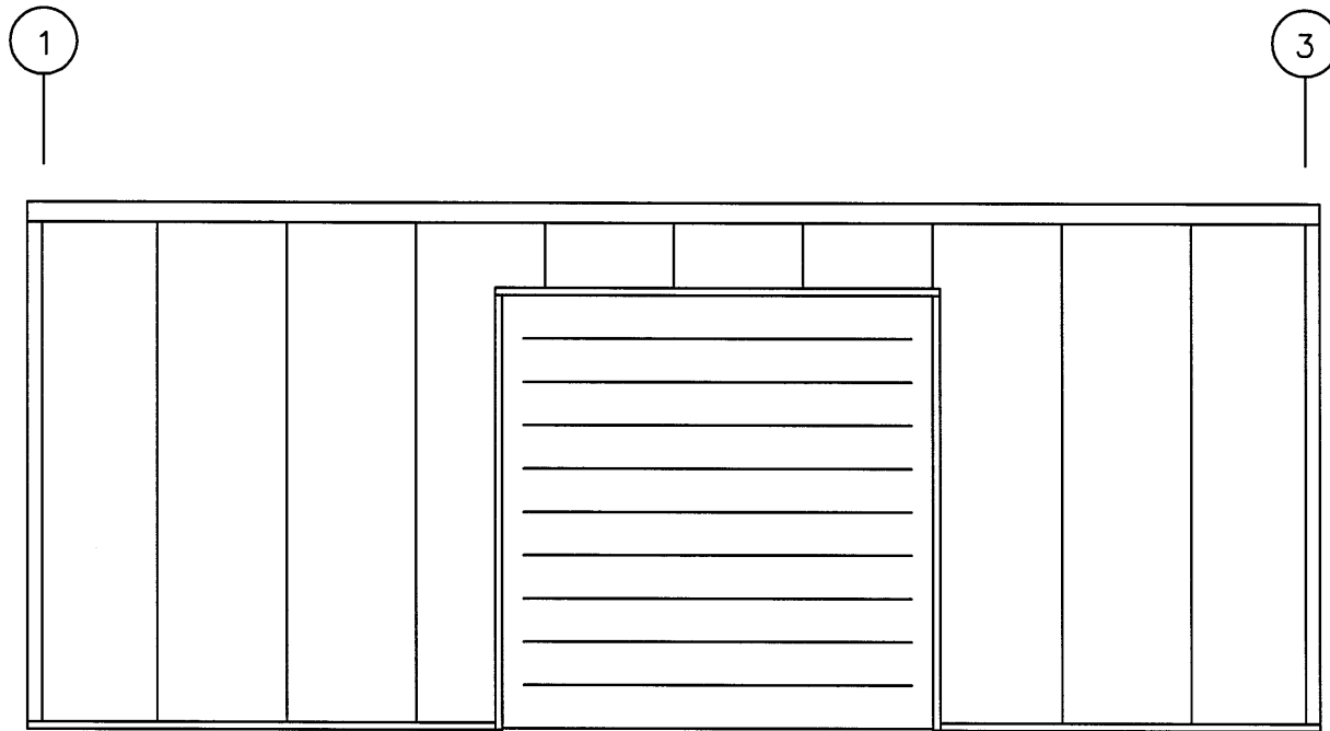
SIDEWALL SHEETED ELEV. @ COL. LINE A N.T.S.
