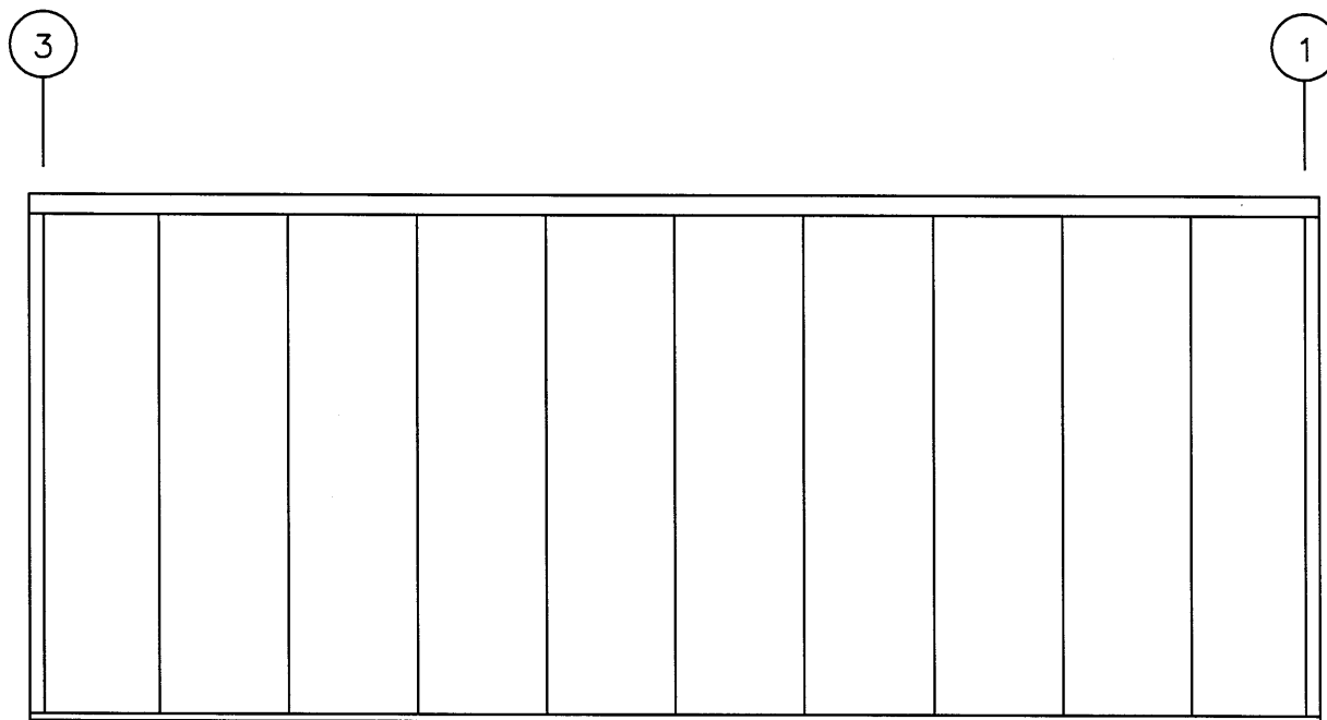
SIDEWALL SHEETED ELEV. @ COL. LINE B N.T.S.
