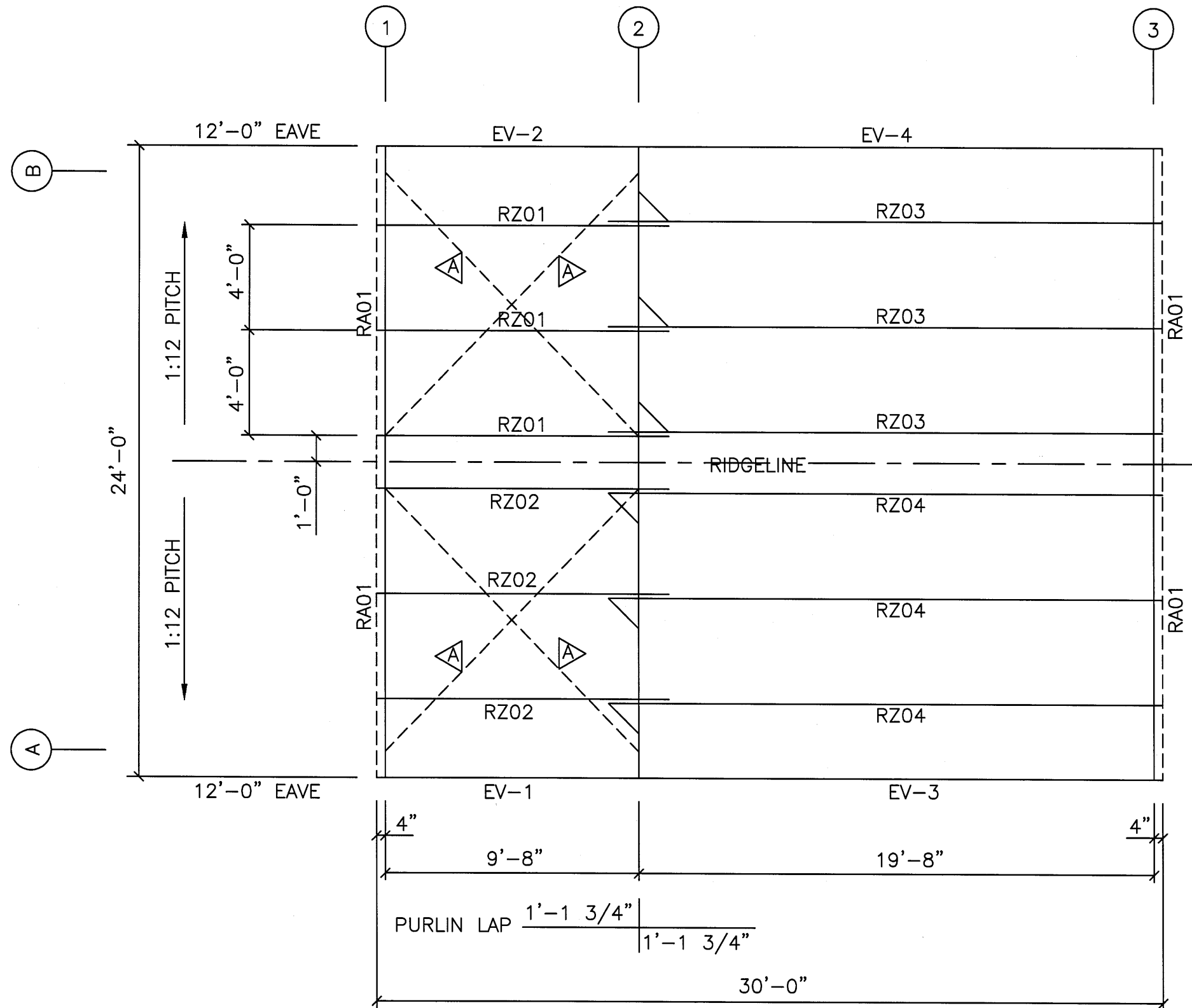
ROOF FRAMING PLAN N.T.S.
