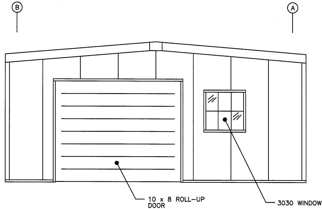
ENDWALL SHEETED ELEV. @ COL. LINE 1 N.T.S.
