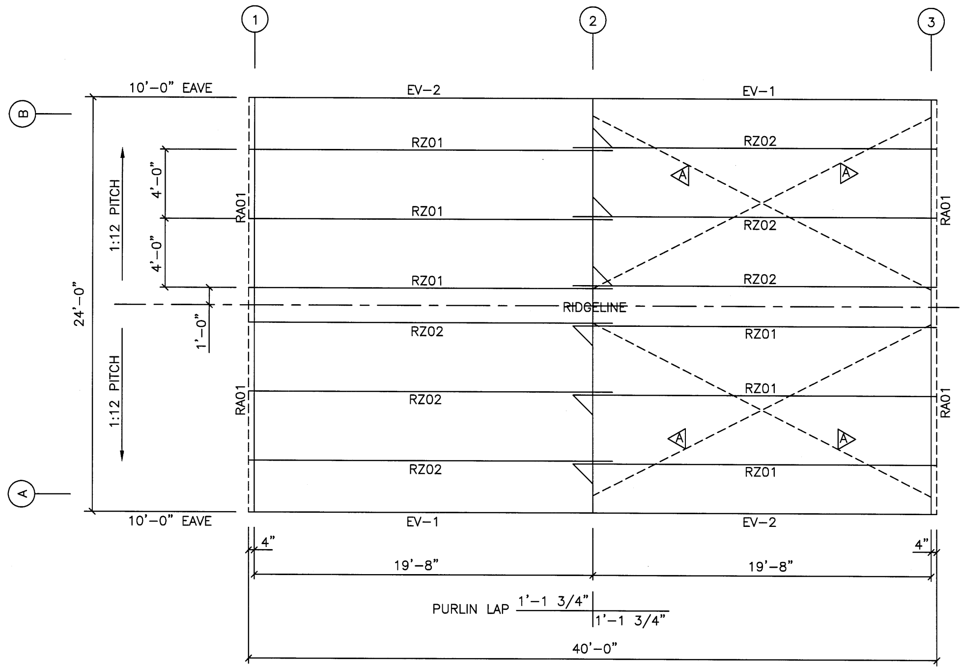
ROOF FRAMING PLAN N.T.S.
