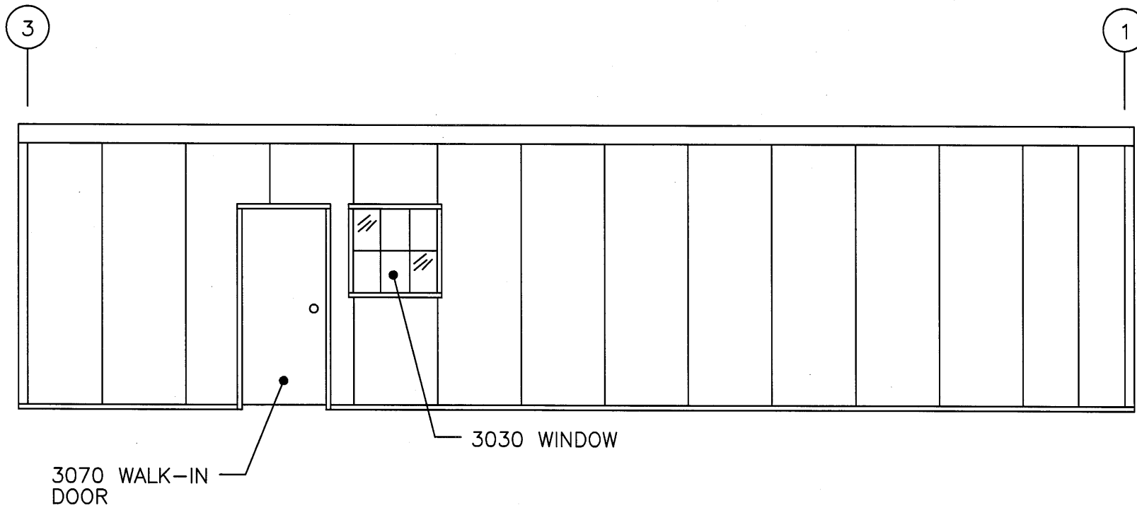
SIDEWALL SHEETED ELEV. @ COL. LINE B N.T.S.
