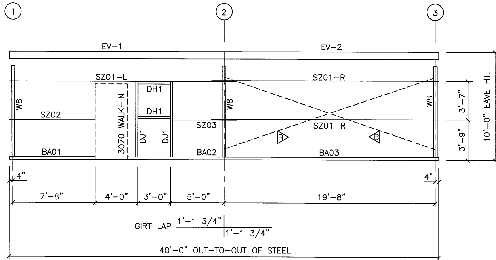
SIDEWALL FRAMING ELEV. @ COL. LINE A N.T.S.
