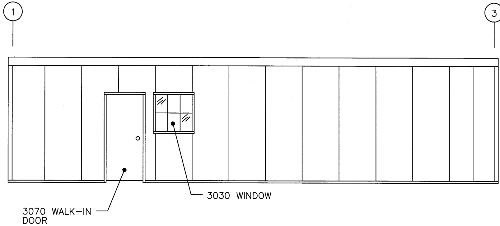
SIDEWALL SHEETED ELEV. @ COL. LINE A N.T.S.
