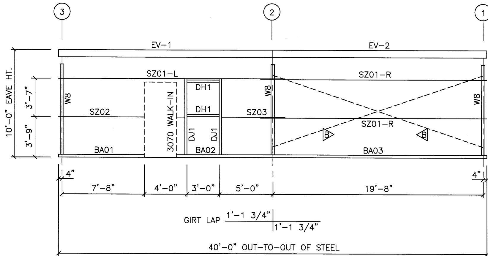
SIDEWALL FRAMING ELEV. @ COL. LINE B N.T.S.
