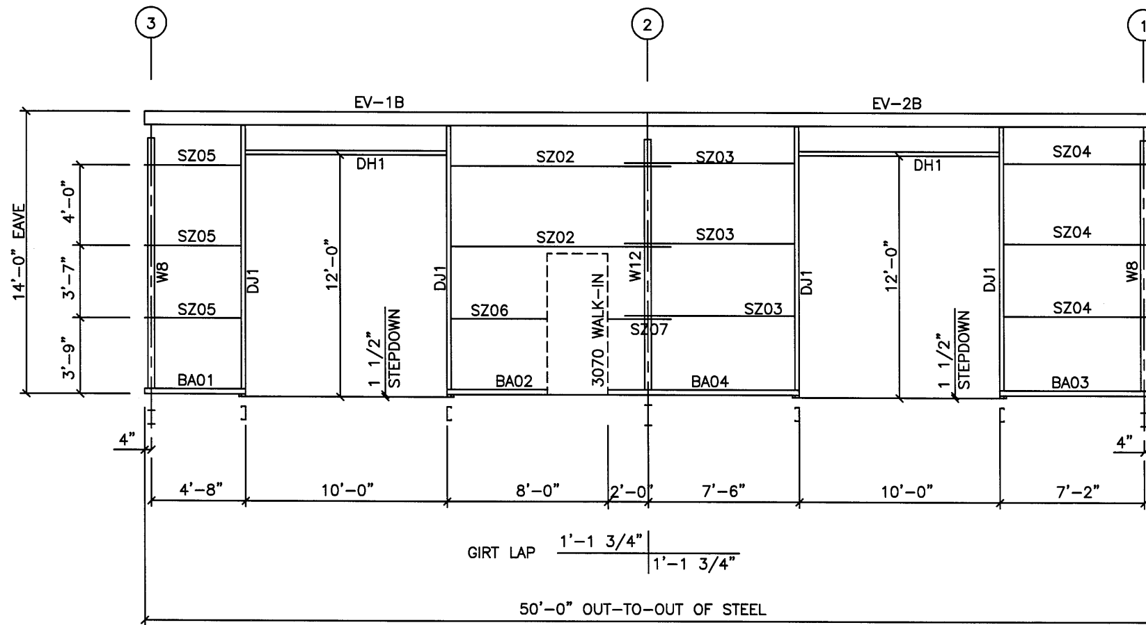
SIDEWALL FRAMING ELEV. @ COL. LINE B N.T.S.
