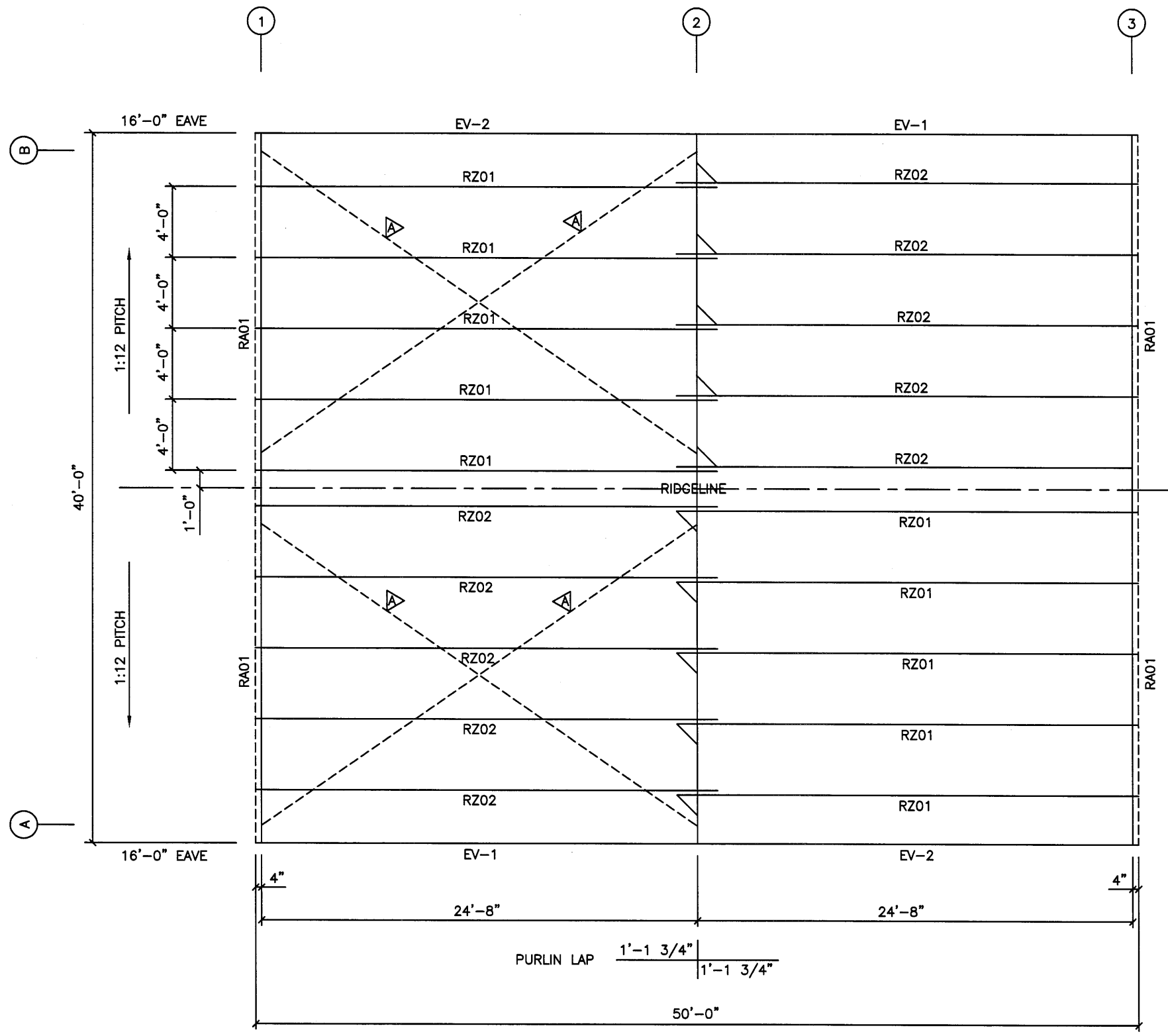
ROOF FRAMING PLAN N.T.S.
