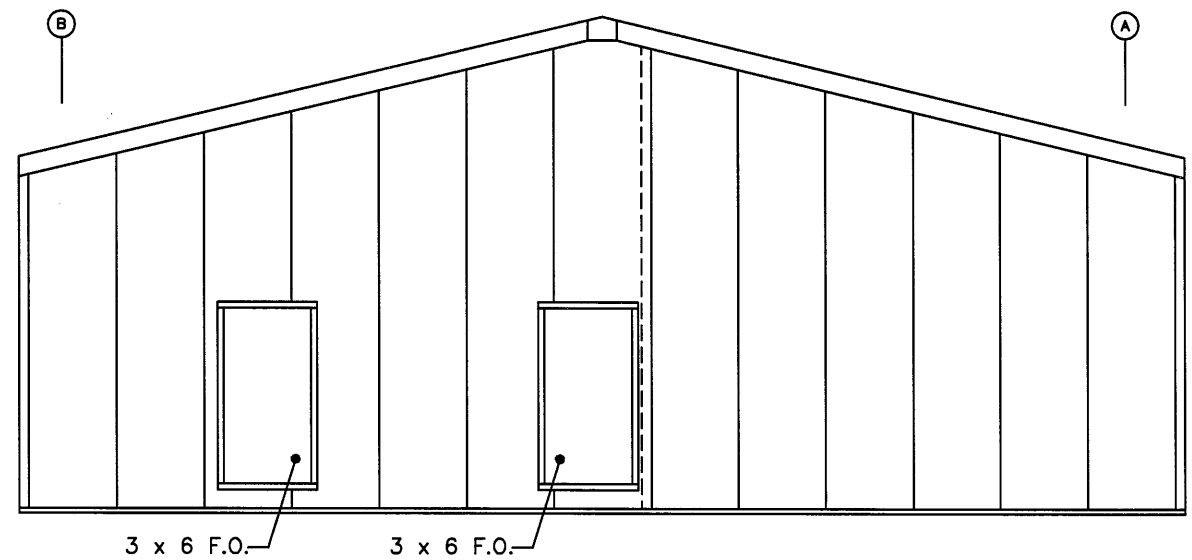
ENDWALL SHEETED ELEV. @ COL. LINE 3 N.T.S.
