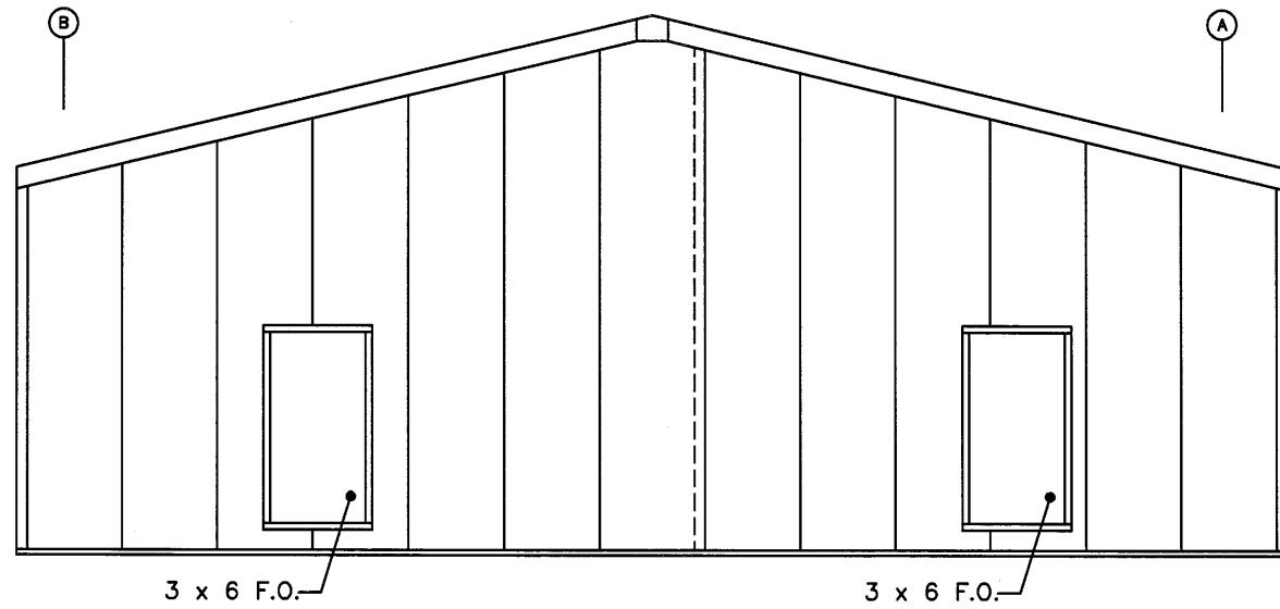
ENDWALL SHEETED ELEV. @ COL. LINE 1 N.T.S.
