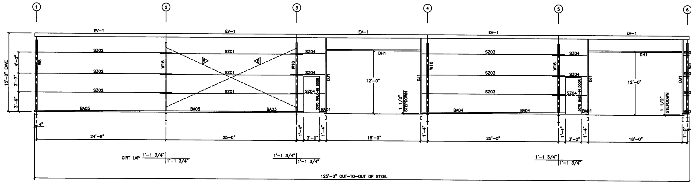
SIDEWALL FRAMING ELEV. @ COL. LINE A N.T.S.
