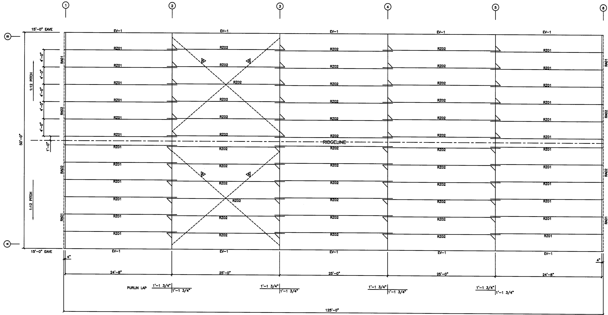
ROOF FRAMING PLAN N.T.S.
