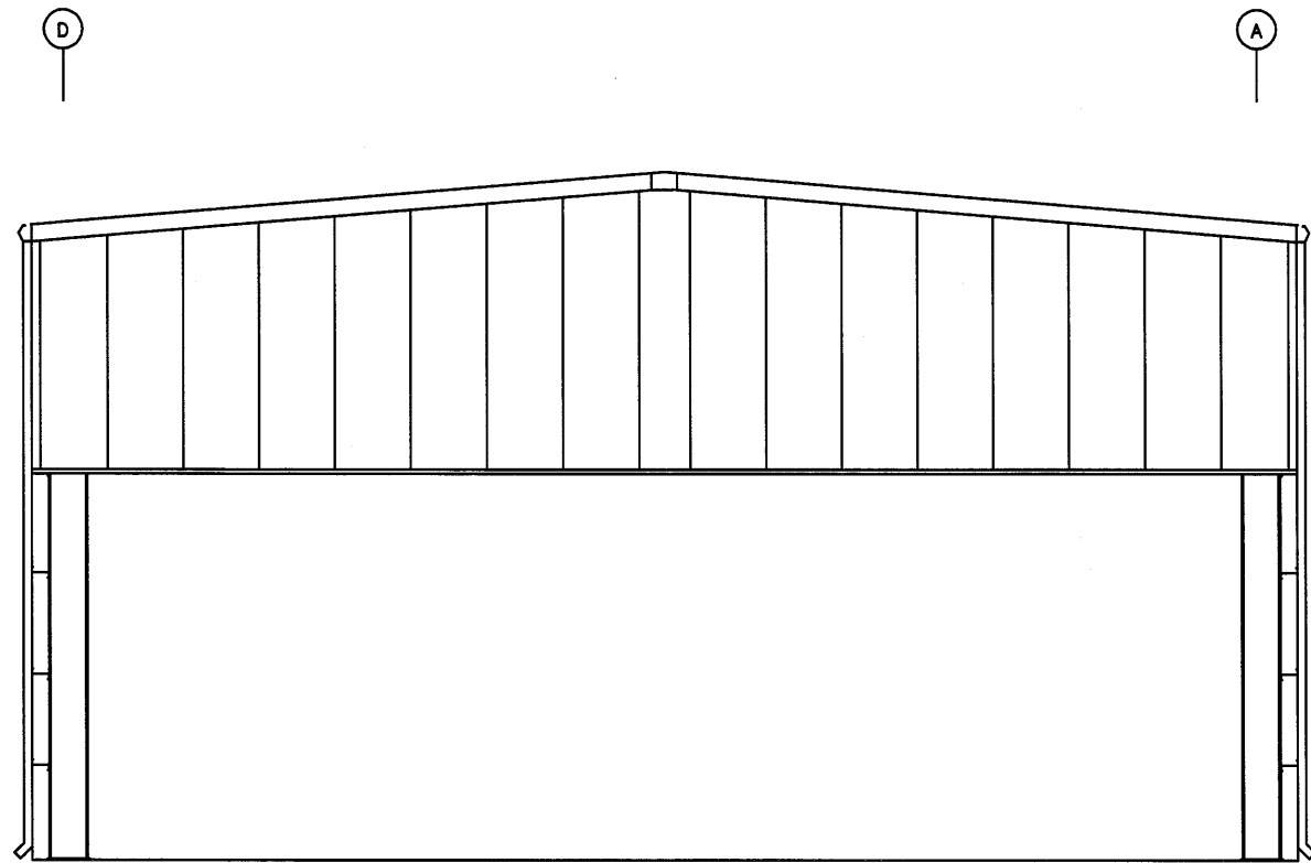
ENDWALL SHEETED ELEV. ● COL. LINE 1 N.T.S.
