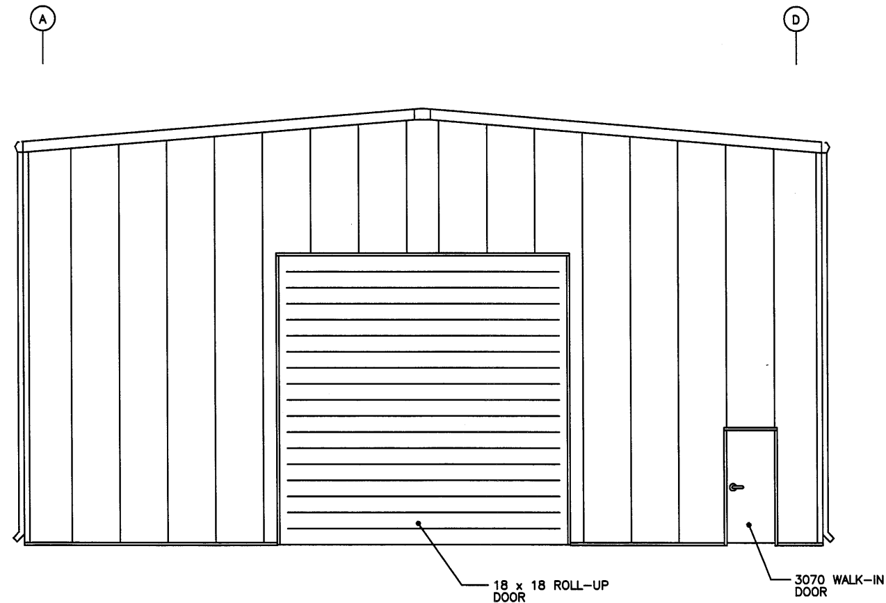
ENDWALL SHEETED ELEV. ● COL. LINE 3 N.T.S.
