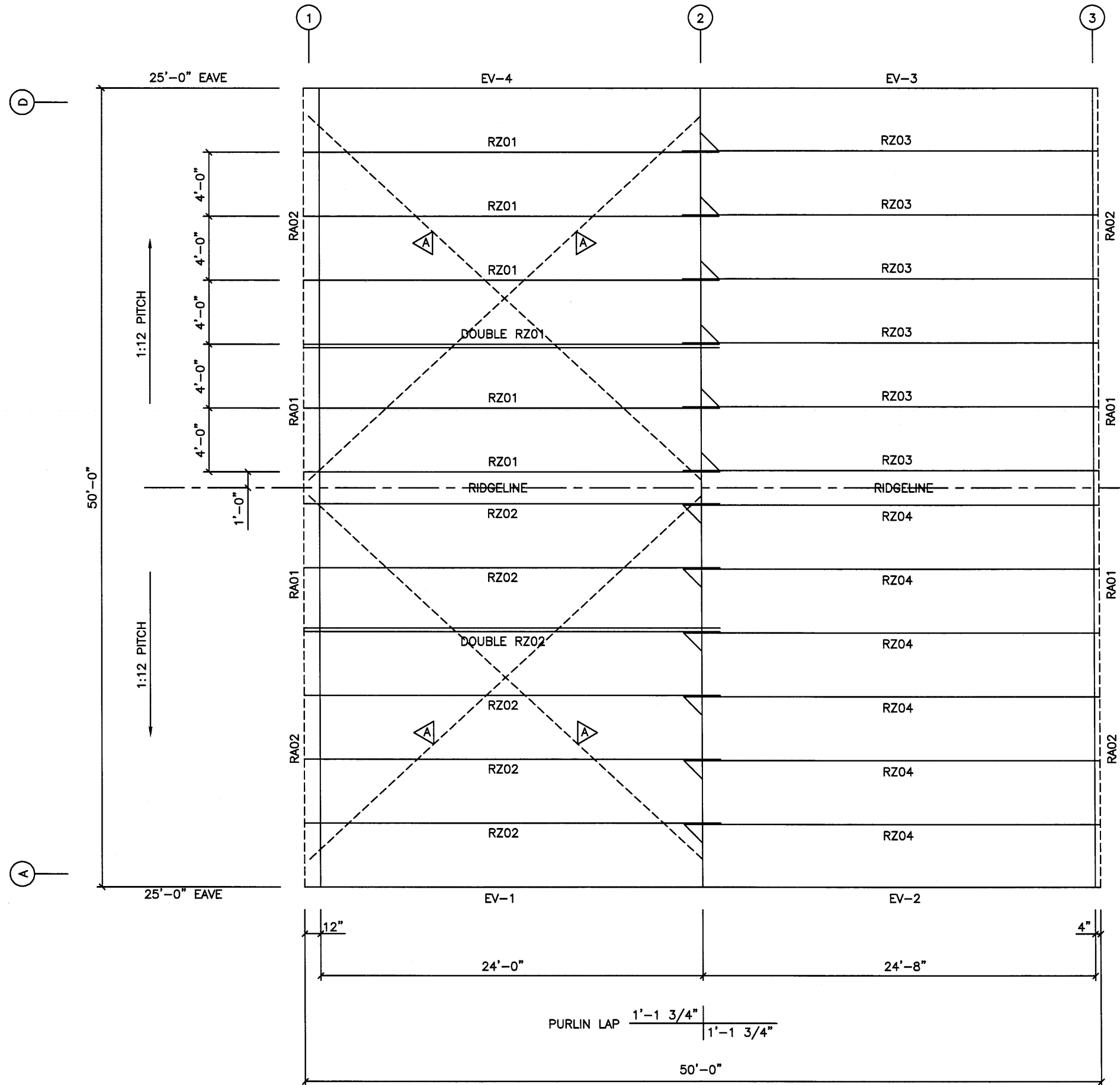
ROOF FRAMING PLAN N.T.S.
