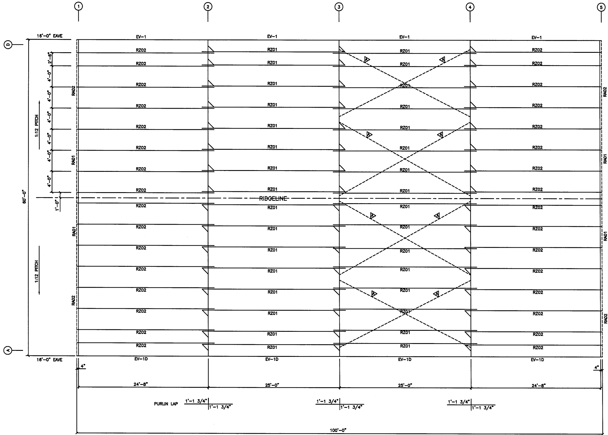
ROOF FRAMING PLAN N.T.S.
