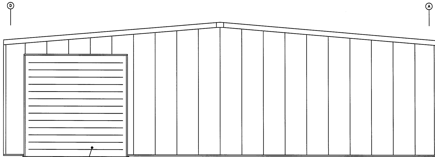
ENDWALL SHEETED ELEV. ● COL. LINE 1 N.T.S.
