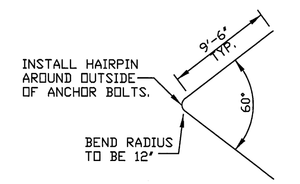
TYPICAL HAIRPIN DETAIL
